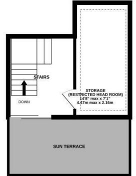
3RD FLOOR 192 sq.ft. (17.9 sq.m.) approx.
